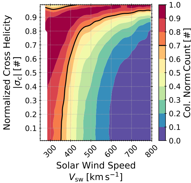
Figure 2. A contour plot of the pdf of |\sigma_c| . The columns in the underlying 2D histogram have been normalized to their maximum value. The contour at 0.7 is indicated in black.
