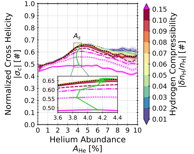
Figure 18. The average normalized cross helicity ( |\sigma_c| ) as a function of the helium abundance ( A_{He} ) in each of 15 compressibility ( |\delta n_H/n_H| ) quantiles. Shaded regions indicate the SEM. The color of each |\delta n_H/n_H| quantile is given by the color bar. Lines are smoothed with a 1\sigma Gaussian filter for visual clarity. Compressibilities |\delta n_H/n_H| > 0.15 are plotted in pink. The quantile corresponding to |\delta n_H/n_H| = 0.085 is highlighted by plotting the dotted orange line on top of a black solid line. The green line plots A_s(|\sigma_c|) in each |\delta n_H/n_H| quantile.
