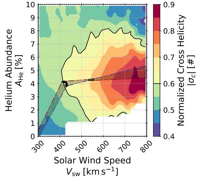
Figure 6. A contour plot of the normalized cross helicity as a function of solar wind speed and helium abundance. The contours are smoothed with a 1\sigma Gaussian filter for clarity. The contour at |\sigma_c| = 0.6 is highlighted in black. The black points mark the saturation point ( v_s, A_s ). The saturation points occur at |\sigma_c| > 0.6 . The shaded black region corresponds to fits to A_{\text{He}}(v_{\text{sw}}) for each |\sigma_c| quantile: the red dashed-dotted line is the high- |\sigma_c| edge, and the blue dashed-dotted line is the low- |\sigma_c| edge. The region from 530 to 560 \text{ km s}^{-1} is where the maximum and minimum |\sigma_c| fits to A_{\text{He}}(|\sigma_c|) cross. This region is bounded by solid black lines and crosses the |\sigma_c| = 0.7 contour.
