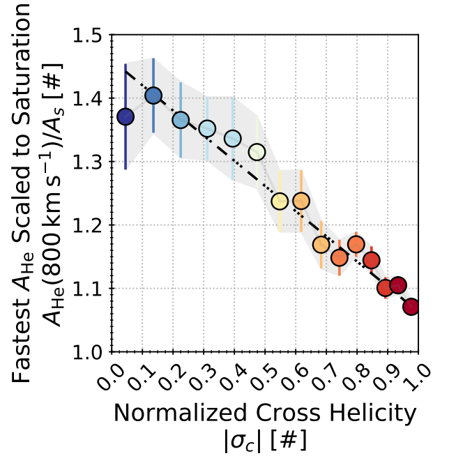
Figure 25. Helium abundance at 800 \text{ km s}^{-1} derived from the fits of A_{\text{He}}(v_{\text{sw}}) across |\sigma_c| quantiles in Paper I, each scaled to the saturation abundance A_s in that paper. Error bars and markers are colored by |\sigma_c| to facilitate comparison with prior figures. The dashed-dotted line is a fit to the trend.
