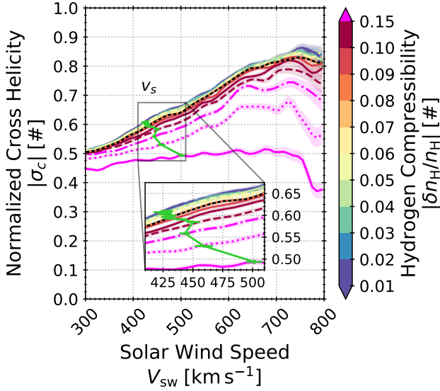
Figure 19. The normalized cross helicity as a function of v_{sw} in the 15 |\delta n_H/n_H| quantiles. Style matches Figure 18, with the green line indicating v_s instead of A_s .
