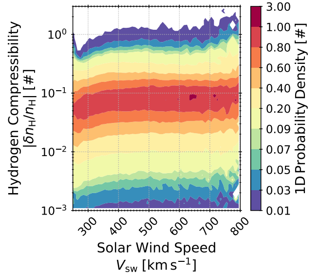
Figure 4. A contour plot of the pdf of |\delta n_H/n_H|(v_{sw}) . In the underlying 2D histogram, the frequency of observing |\delta n_H/n_H| in each column is normalized to its maximum value. The contours are smoothed with a 1\sigma Gaussian kernel for visual clarity.
