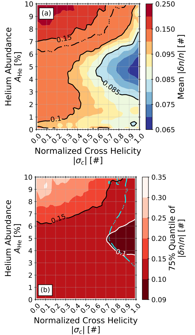
Figure 17. Contour plots of (a) mean and (b) 75% quantile |\delta n_H/n_H| as a function of |\sigma_c| and A_{He} . Contours are smoothed with a 1\sigma Gaussian kernel for visual clarity. Solid black contours in panel (a) indicate |\delta n_H/n_H| = 0.085, 0.1 , and 0.15 . The dashed-dotted black contour indicates where the 75% quantile of |\delta n_H/n_H| = 0.15 in panel (b). Solid contours in panel (b) indicate where the 75% quantile of |\delta n_H/n_H| = 0.1 and 0.15 . The region of the plane with |\sigma_c| greater than that indicated by the dashed-dotted blue line corresponds to solar wind originating in continuously open source regions as defined in Paper I.
