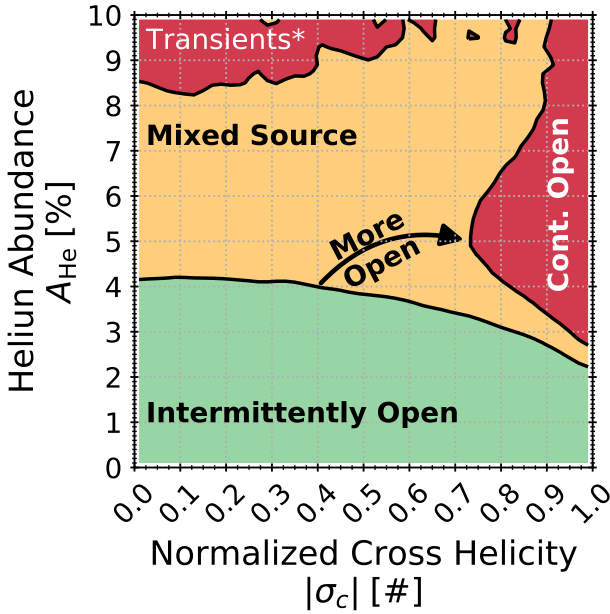
Figure 3. A plot of v_{sw} as a function of |\sigma_c| and A_{He} with contours at v_{sw} = 300 and 460 \text{ km s}^{-1} . Paper I considers helium-poor solar wind with A_{He} < A_r to originate in intermittently open source regions and Alfvénic solar wind with |\sigma_c| > 0.7 in the red region to originate in continuously open source regions. That work hypothesizes that the speed enhancement of non-Alfvénic, helium-rich solar wind in the upper left corner of the plot is due to transients.
