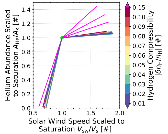
Figure 10. Fits to A_{\text{He}}(v_{\text{sw}}) in 15 |\delta n_{\text{H}}/n_{\text{H}}| quantiles. Each fit is scaled to its situation point ( v_s, A_s ), which is indicated at (1, 1) in green. As in Figure 9, the quantiles are indicated by the color bar.
