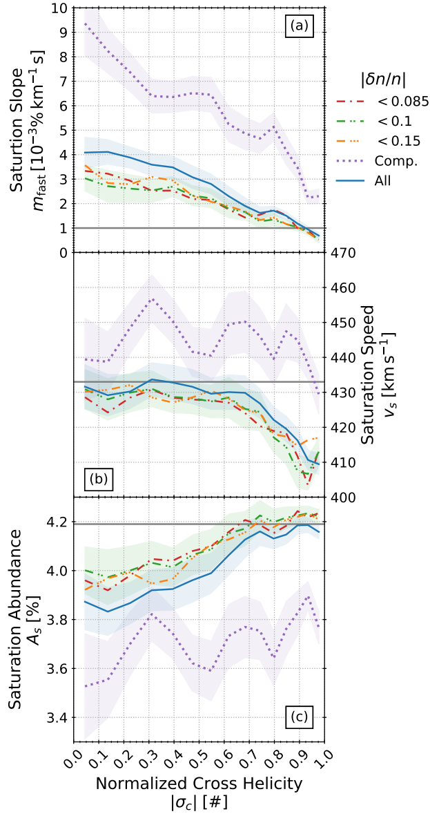
Figure 13. Saturation fit parameters for different maximum |\delta n_H/n_H| , given by the legend, as a function of |\sigma_c| along with the data, irrespective of |\delta n_H/n_H| . The panels are saturation (a) slope ( m_s ), (b) speed ( v_s ), and (c) abundance ( A_s ). Gray lines are the fit parameters across all observations in Figure 1. The “Comp.” subset is compressible solar wind with |\delta n_H/n_H| > 0.15 .
