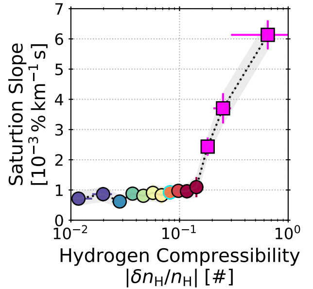
Figure 12. The slopes of A_{He}(v_{sw}) for speeds v_{sw} > v_s in each |\delta n_H/n_H| quantile. Nominally, this is the slope for the fast solar wind originating in open solar wind regions and we refer to them as “saturation slopes” in this work. Quantiles for which |\delta n_H/n_H| > 0.15 are plotted in pink and indicated with squares instead of circles. The marker indicating the quantile with |\delta n_H/n_H| = 0.085 is blue, while all other quantiles have a black marker edge.
