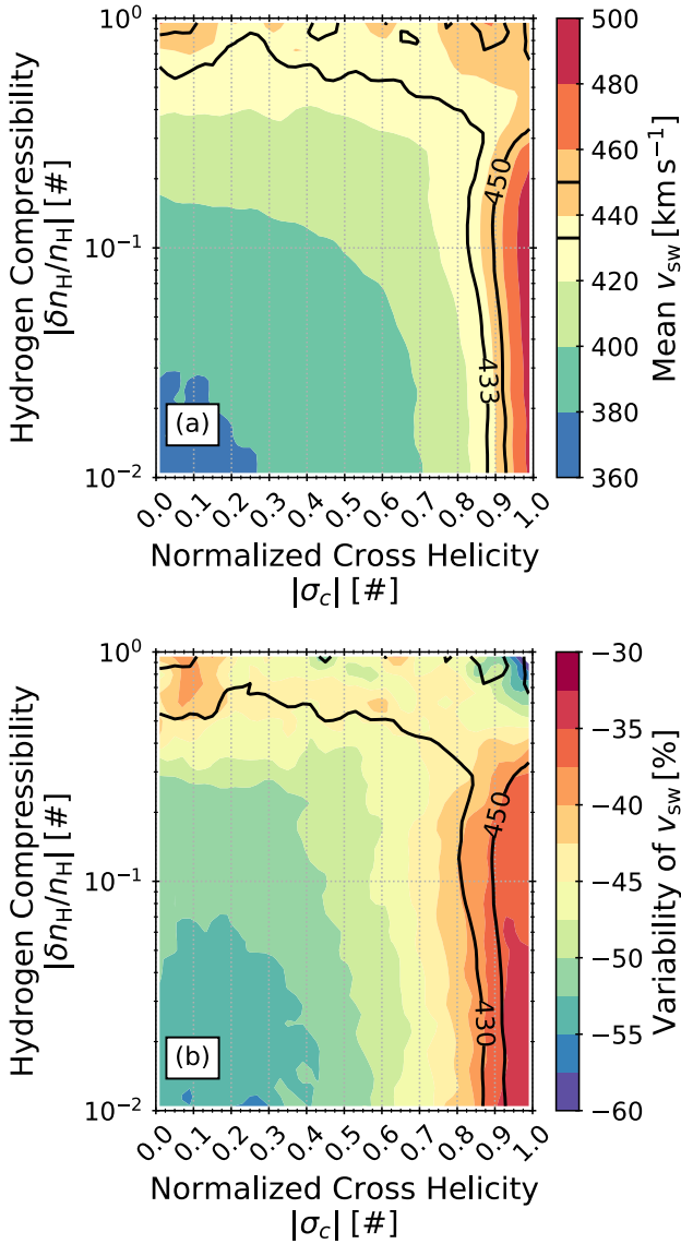
Figure 16. (a) The solar wind speed as a function of cross helicity and compressibility. The black contour indicates v_{sw} = 433 and 450 \text{ km s}^{-1} , the fastest v_s derived in Paper I and for incompressible solar wind ( |\delta n_H/n_H| < 0.15 ) in this work. (b) The variability of v_{sw} calculated in the same manner as in Figure 15.
