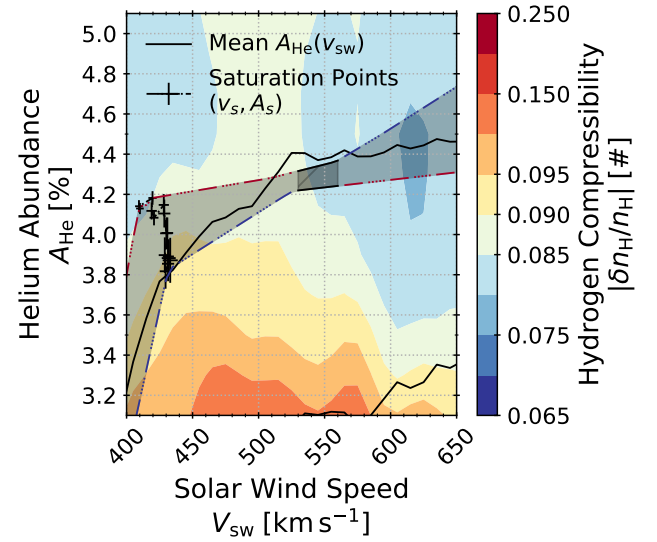
Figure 8. A zoom-in of the region indicated in Figure 7. The gradient of the contour for |\delta n_H/n_H| = 0.09 changes across the saturation points. The fits A_{He}(v_{sw}) cross over the speed range v_{sw} \approx 530 – 560 \text{ km s}^{-1} , which is bounded by solid black lines instead of red and blue dashed-dotted lines. This region where the A_{He}(v_{sw}) fits at low |\sigma_c| become larger than the fits at high |\sigma_c| crosses the |\delta n_H/n_H| = 0.085 contour.
