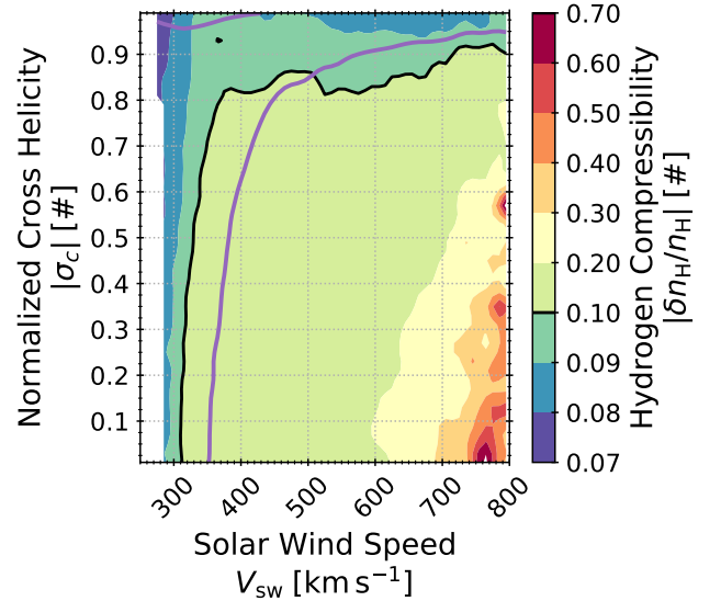
Figure 5. A contour plot of the pdf of |\delta n_H/n_H|(v_{sw}, |\sigma_c|) . Average |\delta n_H/n_H| is calculated as the logarithmic mean. Contours are smoothed with a 1\sigma Gaussian kernel for visual clarity. The purple line is the 0.7 contour from Figure 2.
