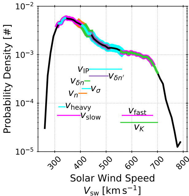
Figure 14. The pdf of the solar wind speed observed by the Wind FCs at 1 au during solar minima 23 and 24 is plotted in black. The colored segments indicate speed ranges derived in this paper, Paper I, B. L. Alterman et al. (2025), and B. Alterman (2025). The v_{sw} range corresponding to each segment is plotted in the same color below the pdf and labeled. The vertical location of these v_{sw} ranges is chosen to avoid overlap. The speed ranges are summarized in Table 4.
