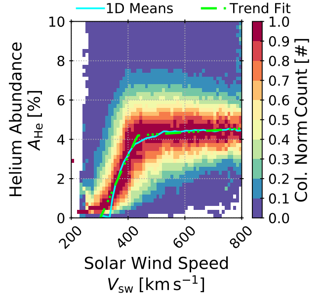
Figure 1. The helium abundance as a function of solar wind speed. A_{He} has been normalized to its maximum value in each column. The blue line indicates the mean value of A_{He} in each column. The dashed–dotted green line is a bilinear fit to these means using Equation (2). The helium abundance monotonically increases from 0% to 4.19% in slow wind and saturates to this A_{He} = 4.19\% in fast solar wind for which v_{sw} > 433 \text{ km s}^{-1} .
