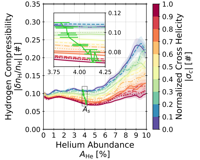
Figure 21. The hydrogen compressibility |\delta n_H/n_H| as a function of the helium abundance A_{He} in quantiles of |\sigma_c| , which is given by the color bar. The green line labeled A_s indicates |\delta n_H/n_H| in each |\sigma_c| quantile at the corresponding saturation abundance.
