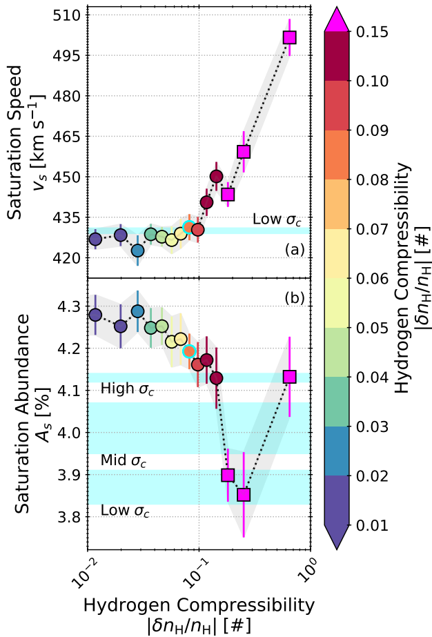
Figure 11. The saturation point ( v_s , A_s ) as a function of |\delta n_H/n_H| . Points are connected by a dotted line to aid the eye. Uncertainties are plotted as error bars with the same color as the markers, and a semitransparent gray envelope traces out the envelope surrounding the error bars. Markers are colored by |\delta n_H/n_H| to facilitate comparison with other figures. As above, quantiles with |\delta n_H/n_H| > 0.15 are shown with pink squares. The edge of the marker corresponding to the quantile for which |\delta n_H/n_H| = 0.085 is blue. The blue horizontal regions correspond to average values of (a) v_s and (b) A_{He} for key ranges of |\sigma_c| derived in Paper I.
