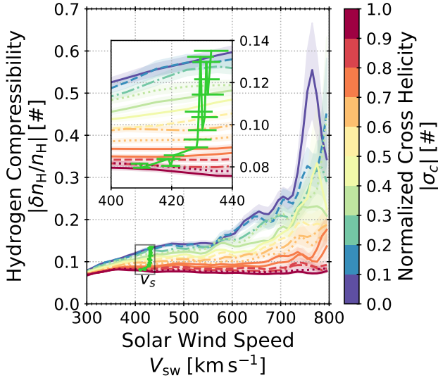
Figure 20. The hydrogen compressibility |\delta n_H/n_H| as a function of the solar wind speed v_{sw} in quantiles of |\sigma_c| , which is given by the color bar. The green line labeled v_s indicates |\delta n_H/n_H| in each |\sigma_c| quantile at the corresponding saturation abundance.
