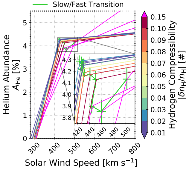
Figure 9. Fits of A_{\text{He}}(v_{\text{sw}}) for 15 quantiles of hydrogen compressibility ( |\delta n_{\text{H}}/n_{\text{H}}| ). The color bar identifies |\delta n_{\text{H}}/n_{\text{H}}| . Quantiles with |\delta n_{\text{H}}/n_{\text{H}}| > 0.15 are indicated in pink. The green plots indicate the saturation points ( v_s, A_s ).
