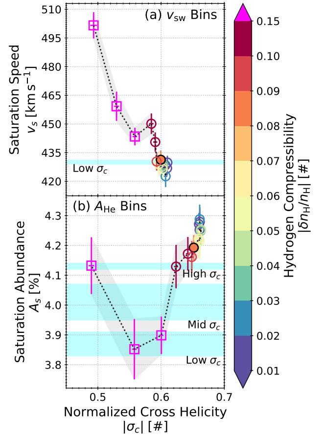
Figure 22. The saturation point (v_s, A_s) in Figure 11 plotted as a function of |\sigma_c| . Points are connected by a dotted line to aid the eye. Uncertainties are plotted as error bars with the same color as the markers, and a semitransparent gray envelope traces out the envelope surrounding the error bars. Each |\delta n_{\text{H}}/n_{\text{H}}| quantile is mapped to |\sigma_c| using (a) Figure 19 and (b) Figure 18. Markers excluding the quantile |\delta n_{\text{H}}/n_{\text{H}}| = 0.085 are open. The |\delta n_{\text{H}}/n_{\text{H}}| = 0.085 quantile marker is filled and has a black edge. As in Figure 11, the blue horizontal regions correspond to the average value of (a) v_s and (b) A_{\text{He}} for key ranges of |\sigma_c| derived in Paper I.
